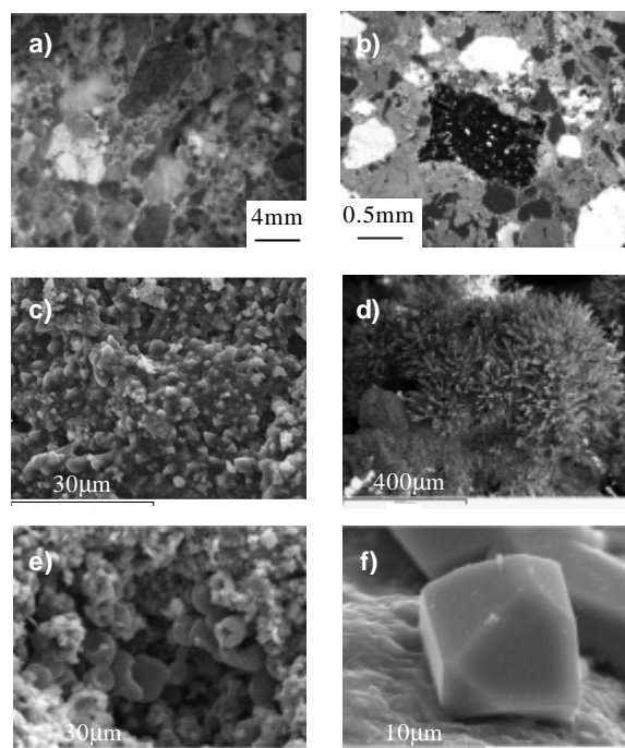
Figure 1. Detail of a) a polished section and of a b) thin-section of the mortars showing crushed ceramics, lime nodules and siliceous sand; SEM micrographs of c) microstructure of a lime matrix d) hydrated calcium silicate crystals growing at the surface of an aggregate, e) biological colonization and f) halite crystal.
